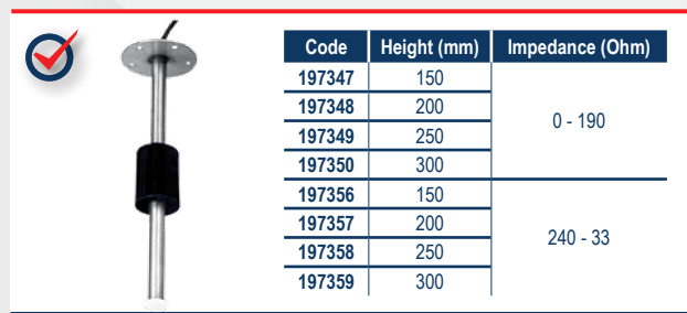
Sensor for Water Tank (12/24V, Inox 316, SAE5)
