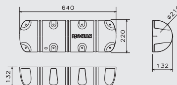
OCEAN Dock Fender 220x640, 1/2, white
