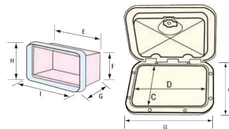
CLASSIC Hatches with Storage Bag ASA - UV resistant
