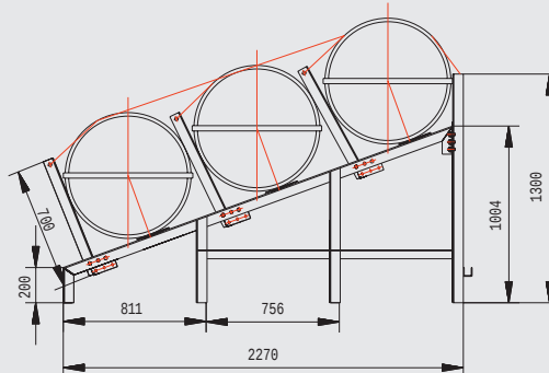
Cradle for SOLAS OCEANO, 3-tier, 6-25(A), 6-35(B)
