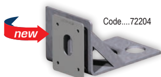
Stern windlass support, SS316, with roller &amp; flange
