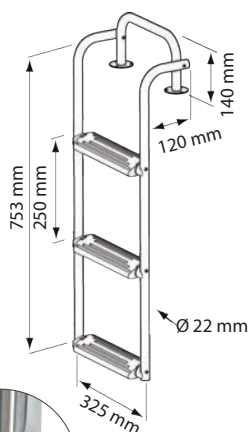
Foldable Ladder,Inox 316, 3 steps 90°- 180°
