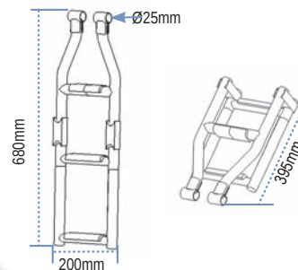
Folding ladder, Inox 316
