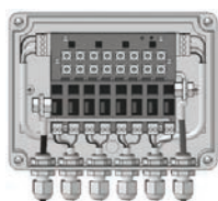
IN/OUT Control Module
