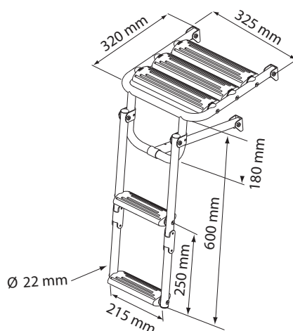
Platform Ladder, Inox 316, with 2 Plastic Steps
