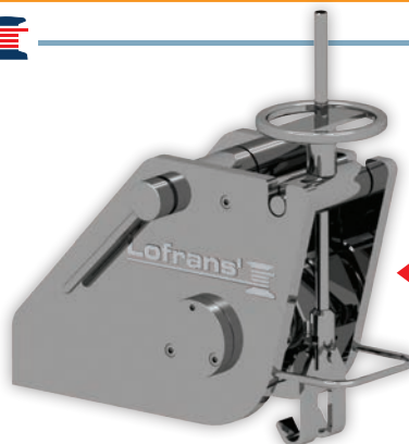
Lofrans' Chain roller-stopper with tensioner, stainless steel, for ISO/DIN/studlink chain 14/16mm
