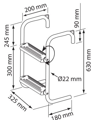
Raft Ladder,Inox 316 2 steps
