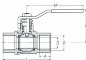
Lever operated ball valve F-F, SeaWare, nickel plated brass, for gas
