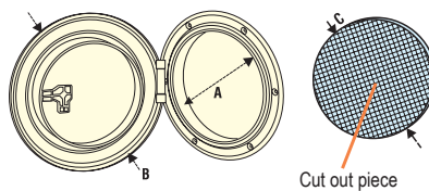
INDUSTRIAL Inspection Hatches PP - UV resistant
