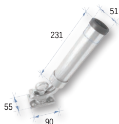
Rod Holder (deck type) Inox 316
